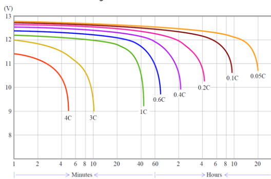
放電曲線 Discharge Characteristics Curves at 25°C
